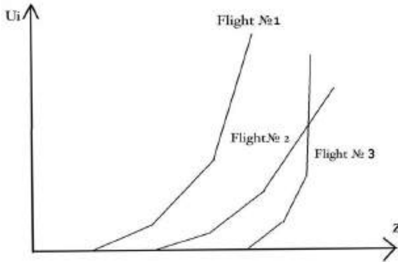
Fig. 1. Dependence of cost losses on the duration of flight delays: z - duration of flight delay, U_i - economic losses.
