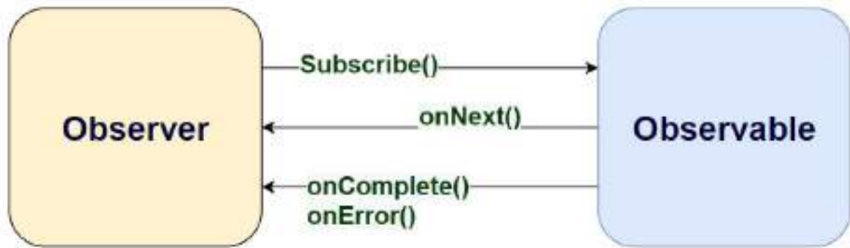
Figure 1. The scheme of patterning Observer
