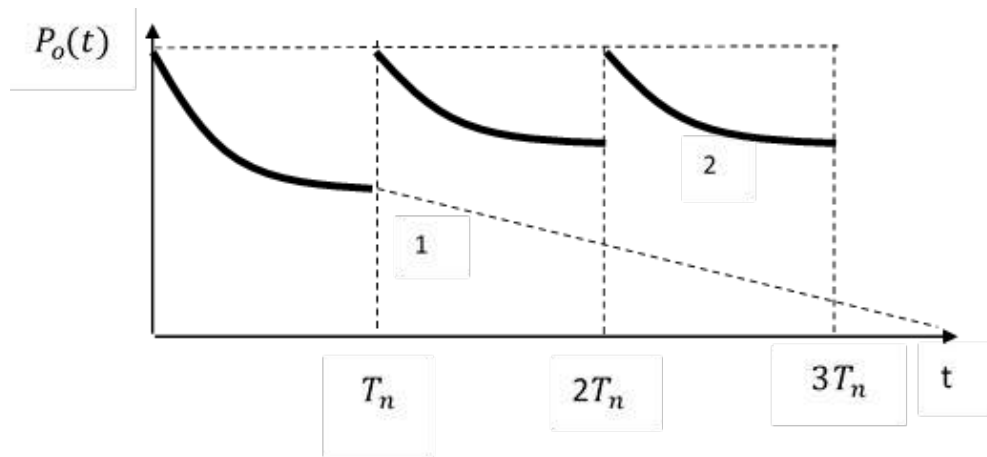
Fig.2. Change in probability of uptime over time: 1 - without preventive maintenance; 2 - with preventive maintenance.
